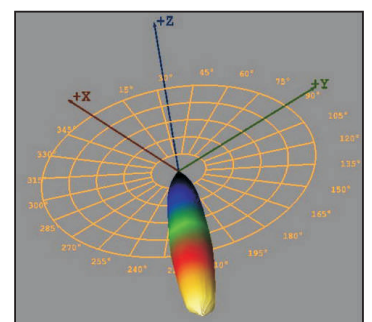
Luminaire light distribution of the 3D
